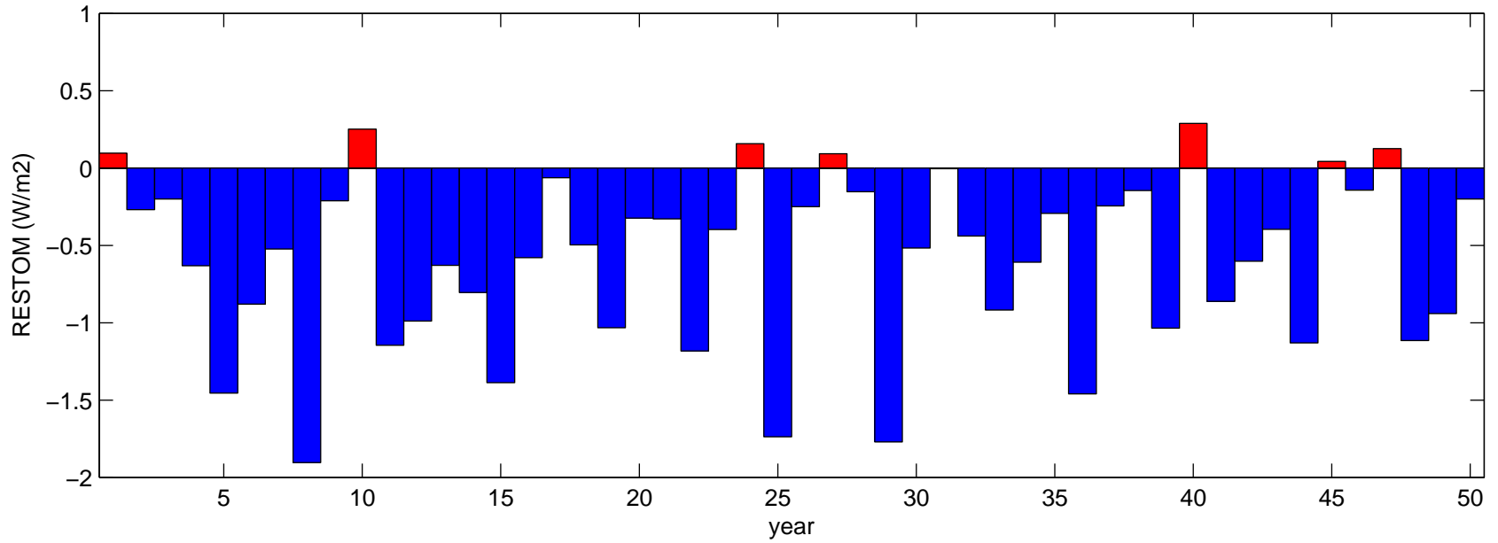
Global Average Top of Atmosphere Energy Balance, MG2 v3
