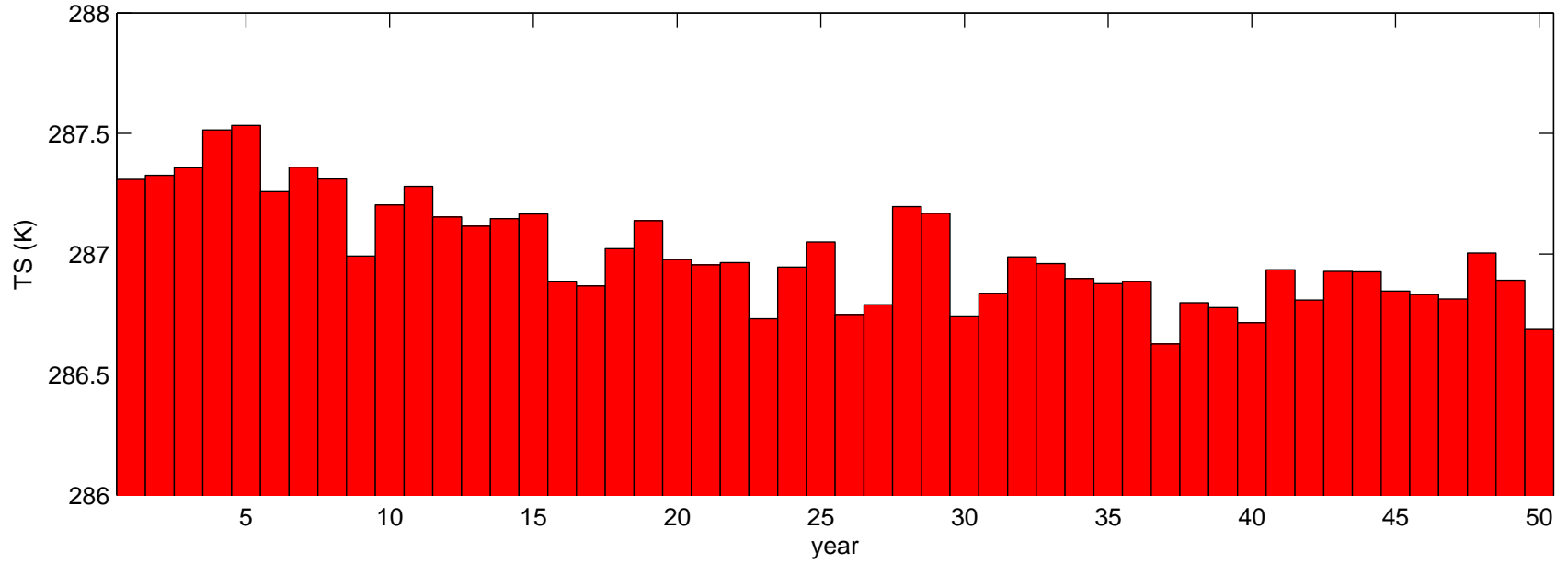
Global Average Surface Temperature, MG2 v3
