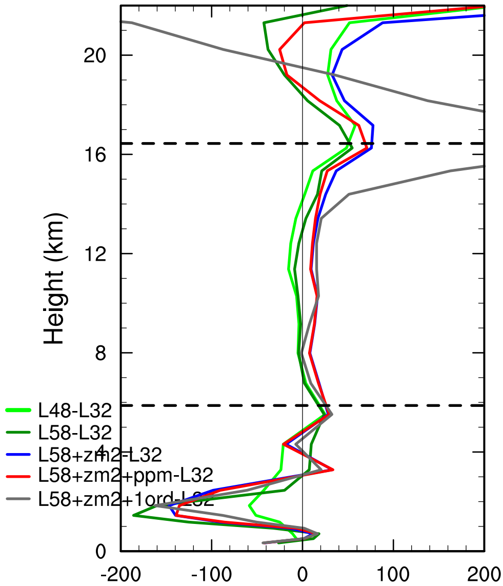
MOISTURE ADVECTION, -OMEGA*dQdp (100*(x-x0)/abs(x0))
