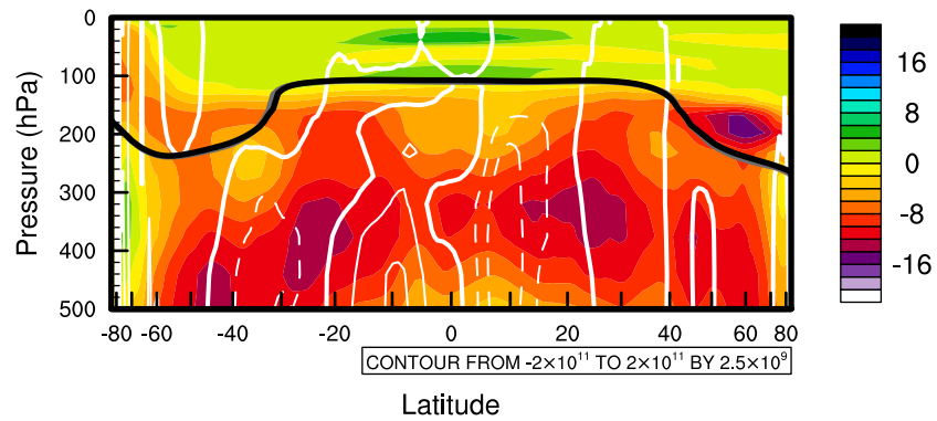
L32(pumas)-L32(cntl) (percent change)
