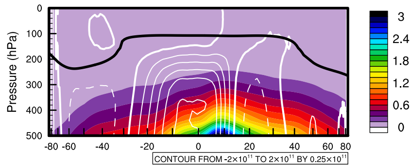
L32(pumas)-L32(cntl) (percent change)
