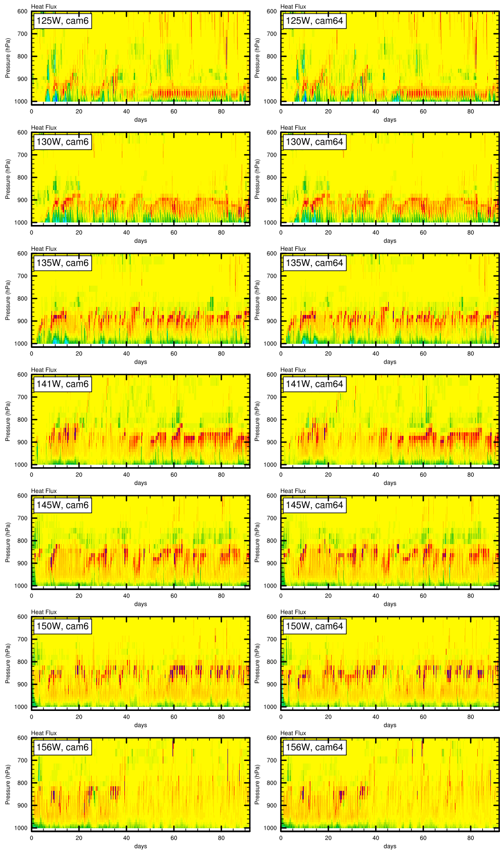
-67.5 -56.25 -45 -33.75 -22.5 -11.25 0 11.25 22.5 33.75 45 56.25 67.5 WPTHLP_CLUBB (W/m 2 )
