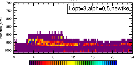
0 0.1 0.2 0.3 0.4 0.5 0.6 0.7 0.8 0.9 1 Fraction plumes with det < 0 & ent > thresh hours
