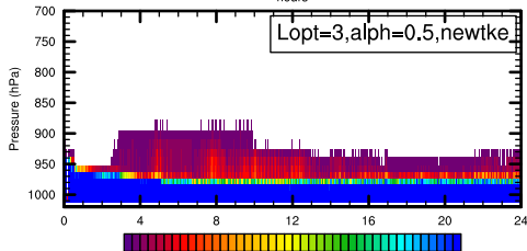
0 7.5 15 22.5 30 37.5 45 52.5 60 67.5 75 82.5 90 97.5 Number of active plumes hours
