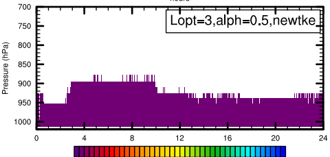
0 0.1 0.2 0.3 0.4 0.5 0.6 0.7 0.8 0.9 1 Fraction plumes det < 0 & ent \leq thresh hours
